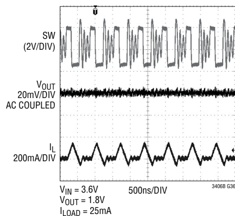
Discontinuous Operation
