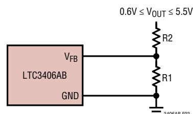
Figure 1. Setting the LTC3406AB Output Voltage
