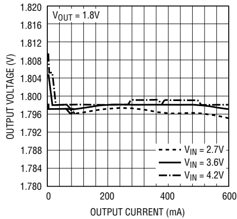
Output vs Load Current
