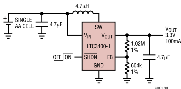
Single Cell to 3.3V Synchronous Boost Converter
