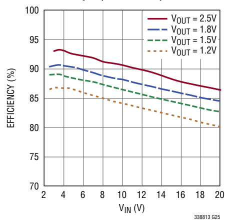
Efficiency vs V_{IN} for I_{LOAD} = 50mA , L = 100\mu H (LTC3388-1)
