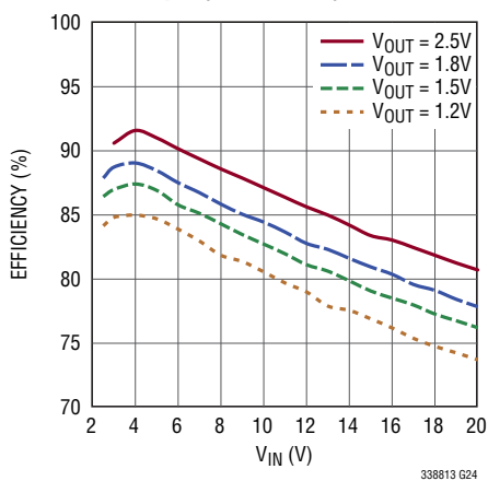
Efficiency vs V_{IN} for I_{LOAD} = 50mA , L = 22\mu H (LTC3388-1)
