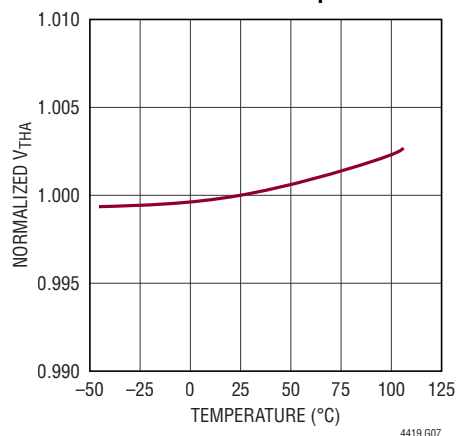
Normalized Falling ADJ Threshold vs Temperature
