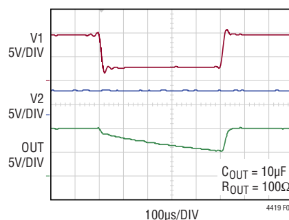
Figure 6. Voltage Waveforms During a Brown-Out on V1 that Does Not Result in a Switchover to V2. Switchover Threshold = 1.8V
