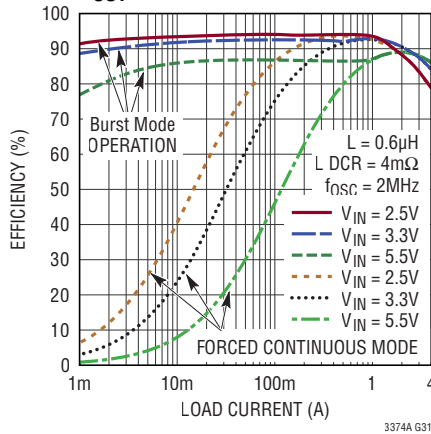
4A Buck Efficiency vs I_{\text{LOAD}} , V_{\text{OUT}} = 1.8\text{V}
