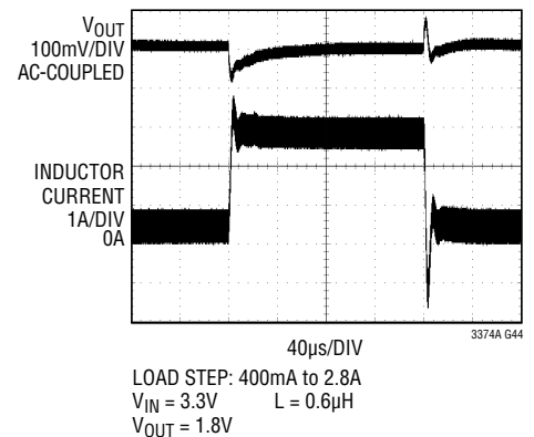
4A Buck Regulator, Transient Response (Forced Continuous Mode)
