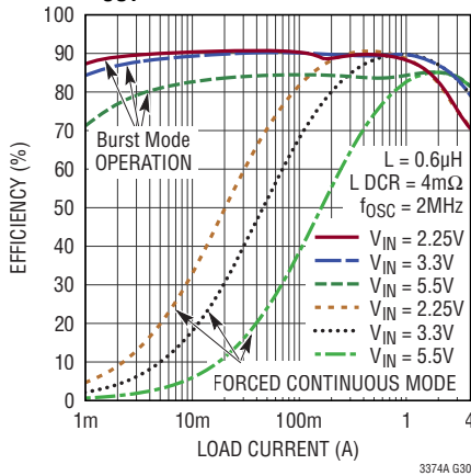
4A Buck Efficiency vs I_{\text{LOAD}} , V_{\text{OUT}} = 1.2\text{V}
