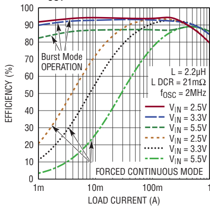
1A Buck Efficiency vs I_{LOAD} , V_{OUT} = 1.8V
