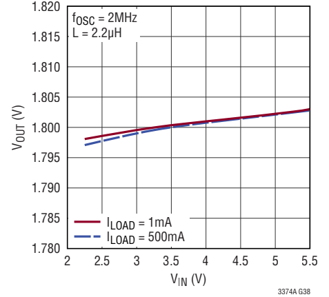
1A Buck Regulator Line Regulation (Forced Continuous Mode)
