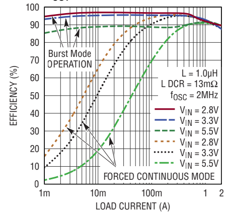
2A Buck Efficiency vs I_{LOAD} , V_{OUT} = 2.5V
