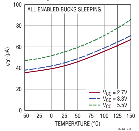
V_{CC} Quiescent Current vs Temperature
