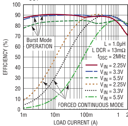
2A Buck Efficiency vs I_{LOAD} , V_{OUT} = 1.2V
