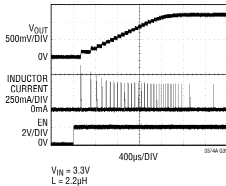
1A Buck Regulator No-Load Start-Up Transient
