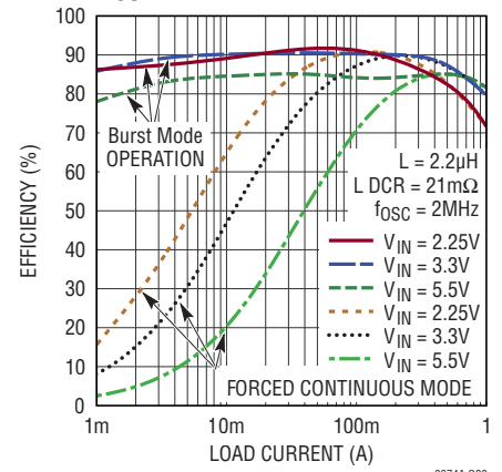
1A Buck Efficiency vs I_{LOAD} , V_{OUT} = 1.2V
