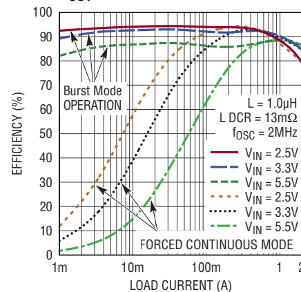
2A Buck Efficiency vs I_{LOAD} , V_{OUT} = 1.8V
