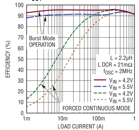
1A Buck Efficiency vs I_{LOAD} , V_{OUT} = 3.3V
