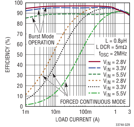
3A Buck Efficiency vs I_{\text{LOAD}} , V_{\text{OUT}} = 2.5\text{V}
