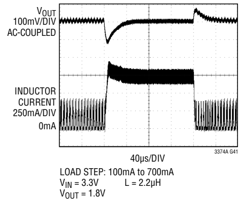
1A Buck Regulator, Transient Response (Burst Mode Operation)
