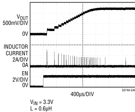
4A Buck Regulator No-Load Start-Up Transient
