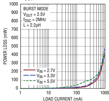
1A Buck Power Loss vs I_{LOAD} , V_{OUT} = 2.5V
