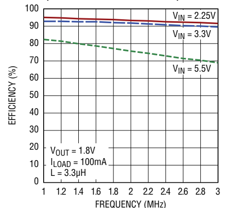
1A Buck Efficiency vs Frequency (Forced Continuous Mode)
