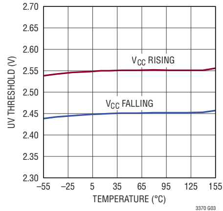
V_{CC} Undervoltage Threshold vs Temperature
