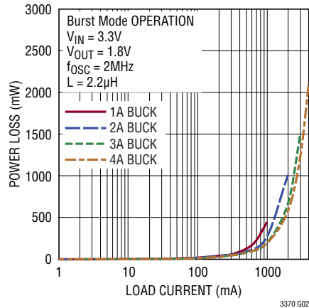
Buck Power Loss vs I_{LOAD}
