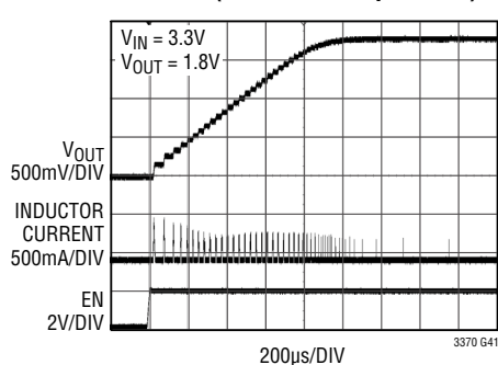
1A Buck Regulator No-Load Start-Up Transient (Burst Mode Operation)
