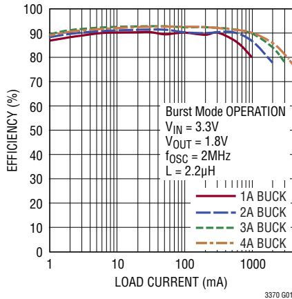
Buck Efficiency vs I_{LOAD}
