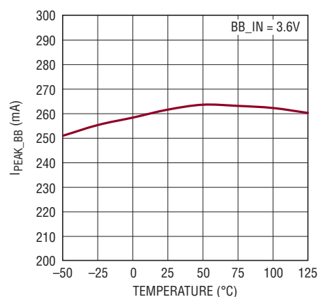
Buck-Boost Peak Current vs Temperature, 250mA I_{PEAK} Setting
