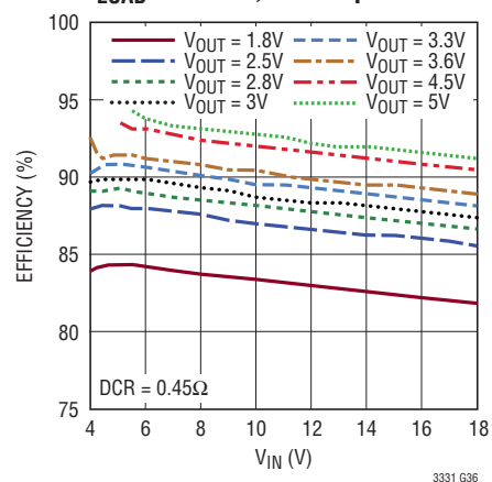
Buck Efficiency vs V IN for I LOAD = 100mA, L = 100μH
