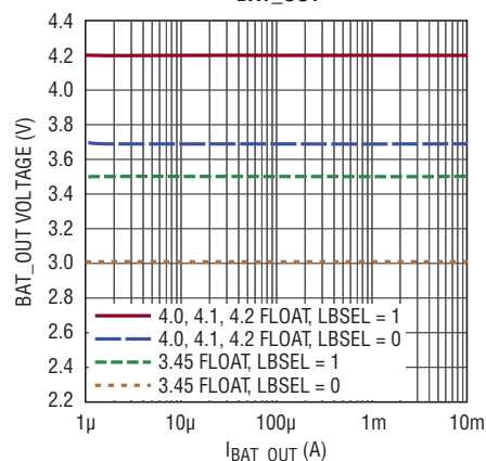
Battery Connect Voltage at BAT_OUT vs I_{BAT\_OUT}
