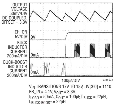
Prioritizer Buck-Boost to Buck Transition
