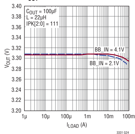
Buck Load Regulation, 3.3V
