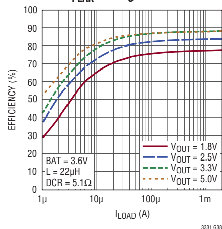
Buck-Boost Efficiency vs I LOAD , 5mA I PEAK Setting
