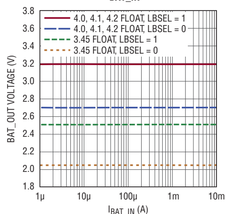
Battery Disconnect Voltage at BAT_OUT vs I_{BAT\_IN}
