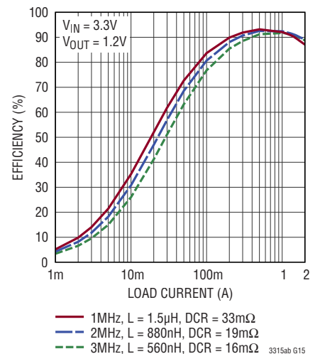
Efficiency vs I_{LOAD} Syncing, Forced Continuous
