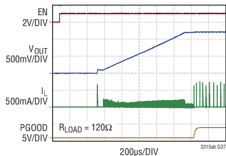
Startup Transient, Burst Mode
