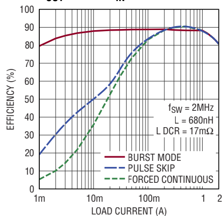
Efficiency vs I_{LOAD} , V_{OUT} = 0.8\text{V} , V_{IN} = 2.25\text{V}
