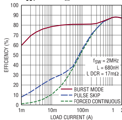
Efficiency vs I_{LOAD} , V_{OUT} = 0.8\text{V} , V_{IN} = 5.5\text{V}
