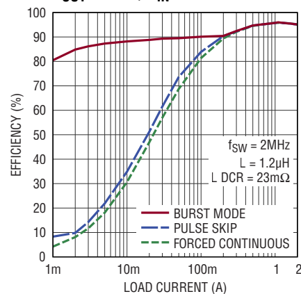
Efficiency vs I_{LOAD} , V_{OUT} = 3.3\text{V} , V_{IN} = 5.5\text{V}
