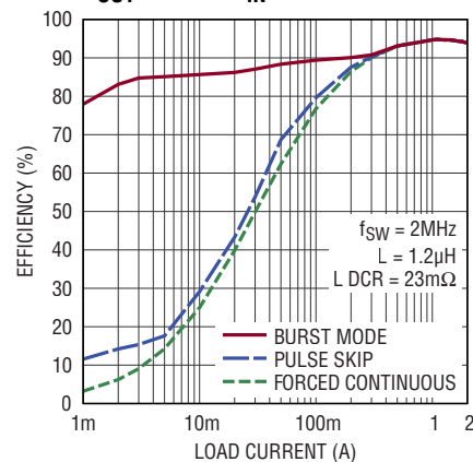
Efficiency vs I_{LOAD} , V_{OUT} = 2.5\text{V} , V_{IN} = 5.5\text{V}
