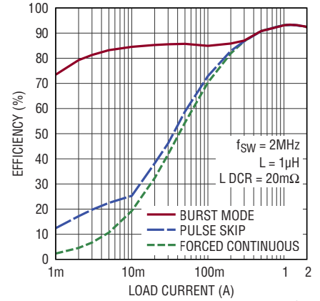
Efficiency vs I_{LOAD} , V_{OUT} = 1.8\text{V} , V_{IN} = 5.5\text{V}
