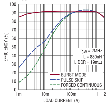
Efficiency vs I_{LOAD} , V_{OUT} = 1.2\text{V} , V_{IN} = 2.25\text{V}
