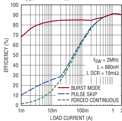
Efficiency vs I_{LOAD} , V_{OUT} = 1.2\text{V} , V_{IN} = 5.5\text{V}
