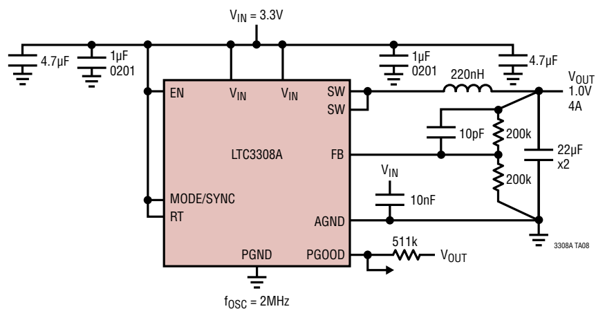
High Efficiency, 2MHz, 4A, 3.3V to 1.0V
