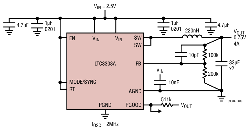
High Efficiency, 2MHz, 4A, 2.5V to 0.75V
