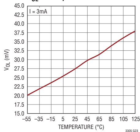
V_{OL} vs Temperature
