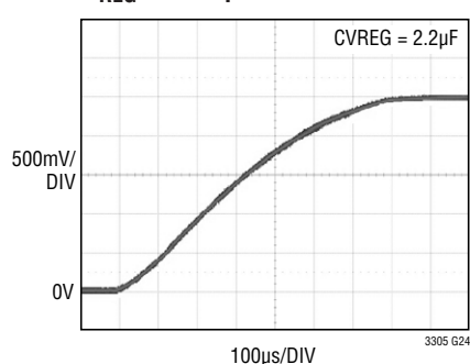
V_{REG} Start-Up
