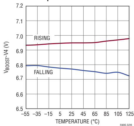
Minimum Boost Voltage vs Temperature
