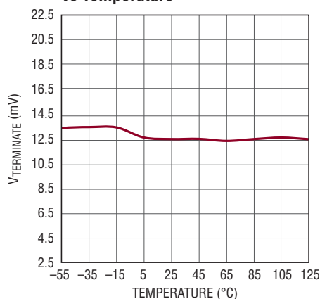
12.5mV Termination Threshold vs Temperature
