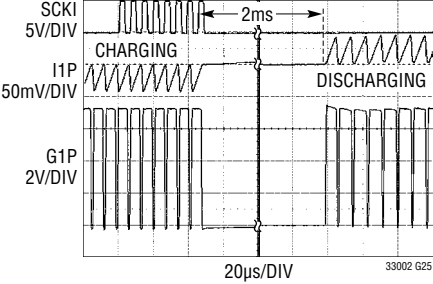
Changing Balancer Direction "On the Fly"
