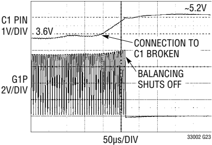
Protection for Broken Connection to Cell While Charging
