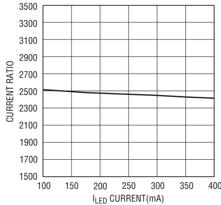
Flash I_{LED}/I_{SET} Current Ratio vs I_{LED} Current (ENT = LOW, ENF = HIGH)
