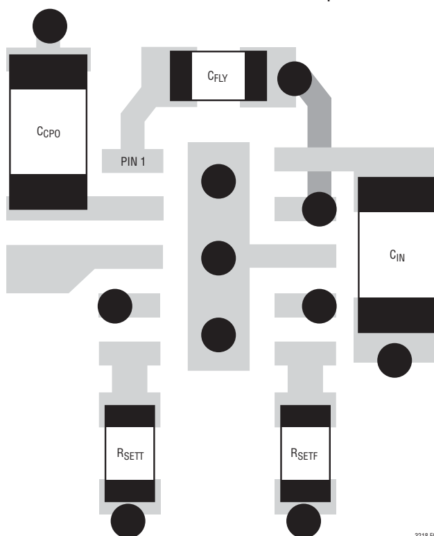
Figure 3. Example Board Layout
