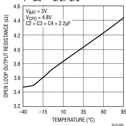
2x Mode Charge Pump Open-Loop Output Resistance vs Temperature
