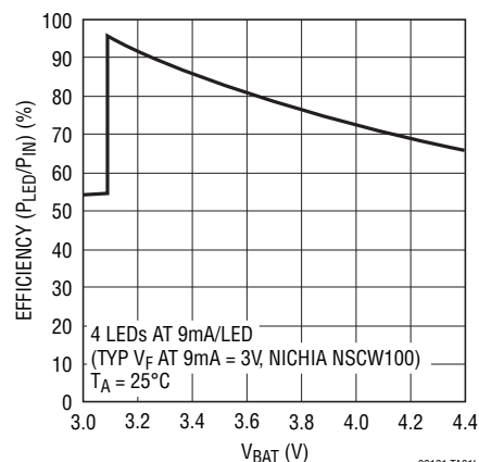
4-LED MAIN Display Efficiency vs V_{BAT} Voltage
