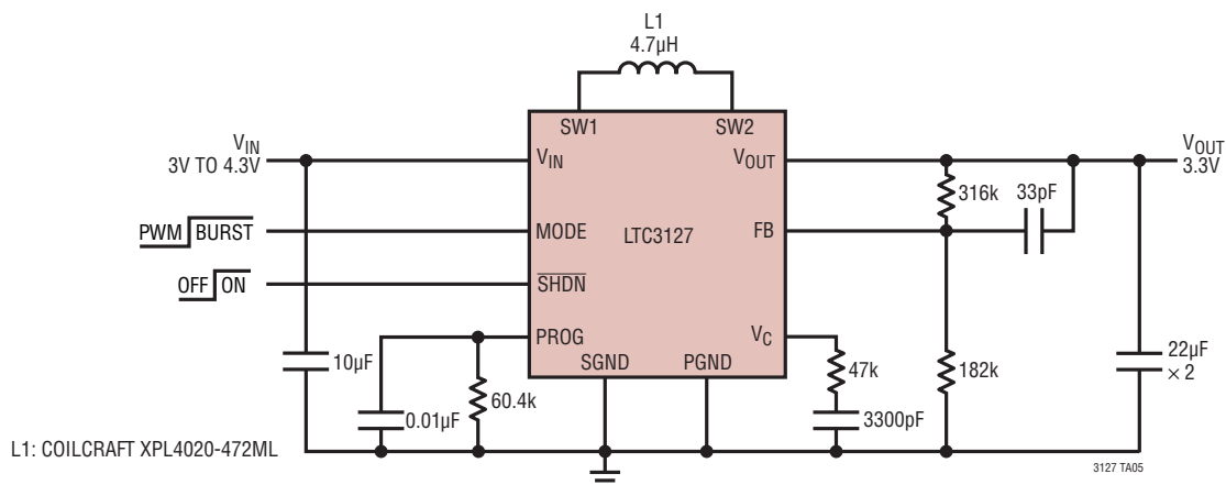
General Purpose Forced Continuous Conduction Application with 500 \mu s Start-Up
