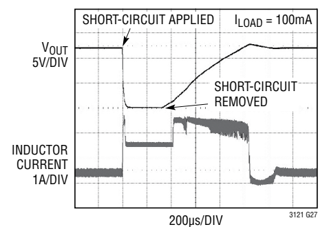
Short-Circuit Response
