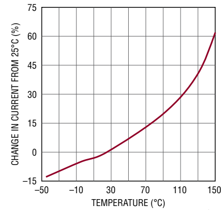
Burst Mode Quiescent Current Change vs Temperature
