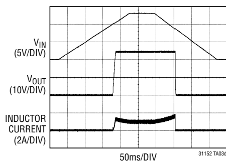
Power-Up/Down Waveforms, I_{LOAD} = 0.5A
