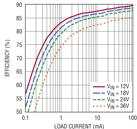
Burst Mode Efficiency, V_{OUT} = 24\text{V} , L = 15\mu\text{H}
