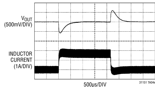
0A to 1.5A Load Step, V_{IN} = 40V
