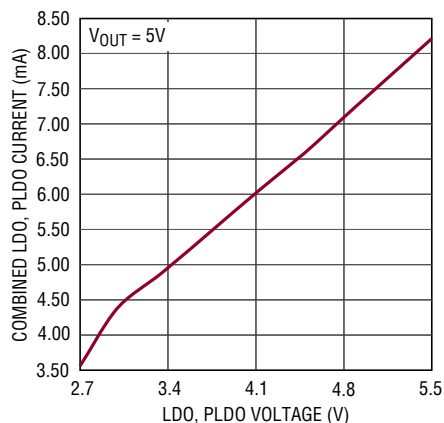
Combined LDO, PLDO Supply Current vs LDO
