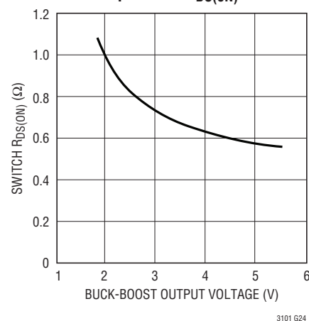
Hot Swap Switch R_{DS(ON)}
