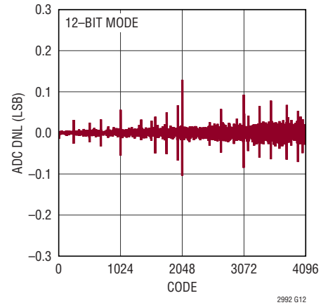
ADC Differential Nonlinearity (GPIO)
