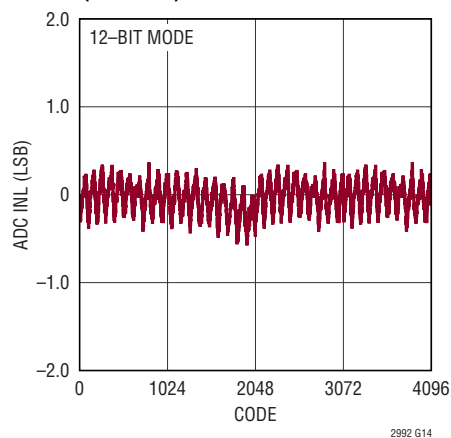
ADC Integral Nonlinearity ( \Delta SENSE)
