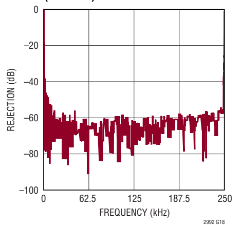
ADC Input Signal Attenuation ( \Delta SENSE)
