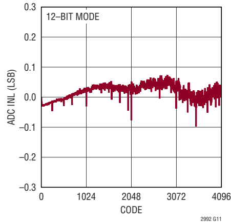
ADC Integral Nonlinearity (GPIO)
