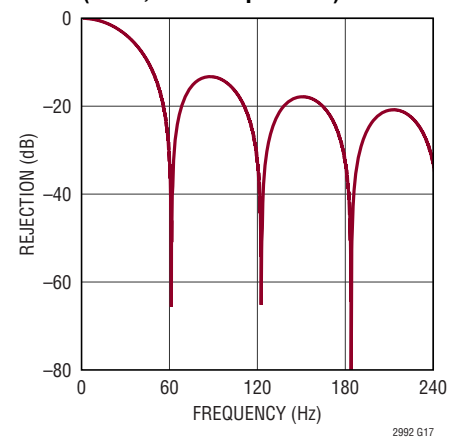
ADC Input Signal Attenuation (GPIO, Low Frequencies)
