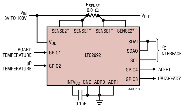
Bidirectional Wide Range Power Monitor
