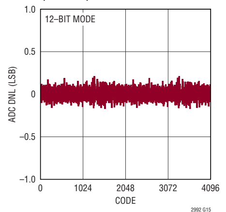
ADC Differential Nonlinearity ( \Delta SENSE)
