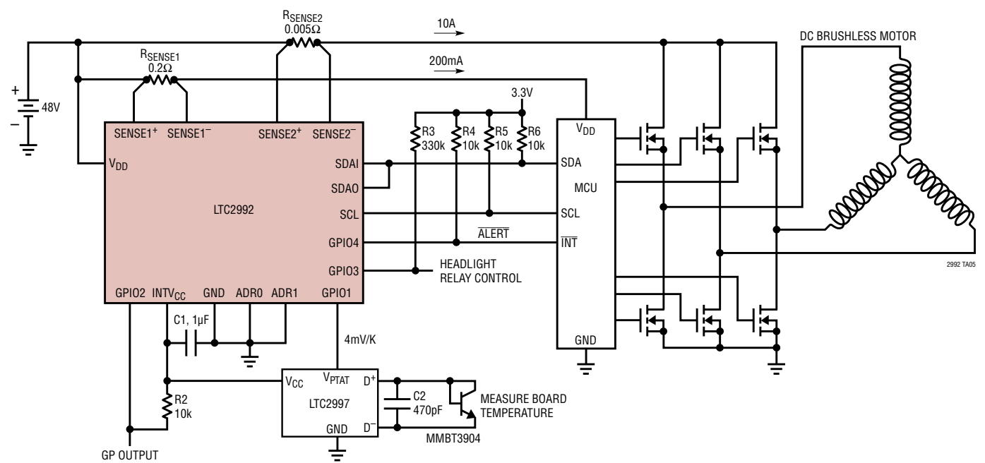
Power Monitor for 48V, 500W Electric Bike/Scooter
