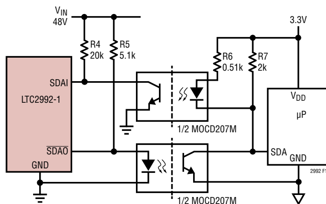
Figure 17. Opto-Isolation of a 1.5kHz I 2 C Interface Between LTC2992-1 and Microcontroller (SCL Omitted for Clarity)
