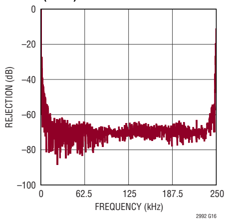
ADC Input Signal Attenuation (GPIO)
