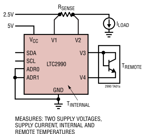
Voltage, Current, Temperature Monitor
