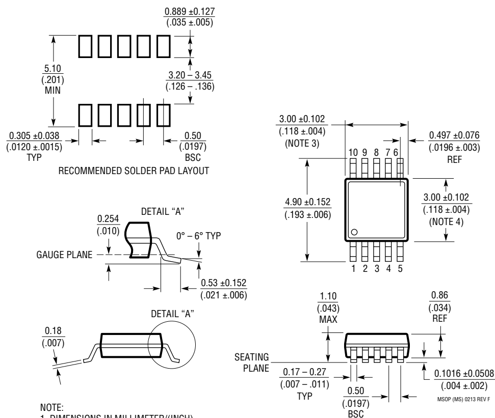
MS Package 10-Lead Plastic MSOP (Reference LTC DWG # 05-08-1661 Rev F)
