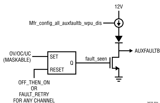
Figure 1. AUXFAULTB MUX
