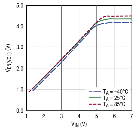
EN Output High Voltage vs Supply Voltage
