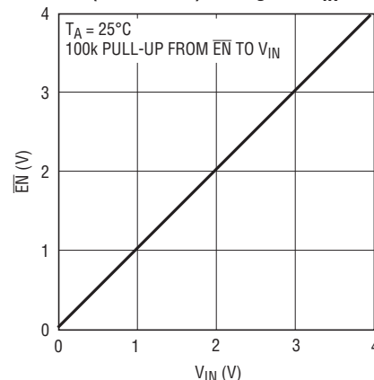
\overline{\text{EN}} (LTC2954-2) Voltage vs V_{\text{IN}}
