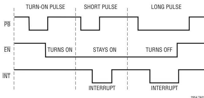
Pushbutton On/Off with Interrupt
