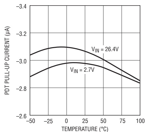
PDT Pull-Up Current vs Temperature
