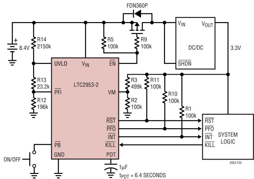
Figure 25. PowerPath Controller with Low Battery Detect
