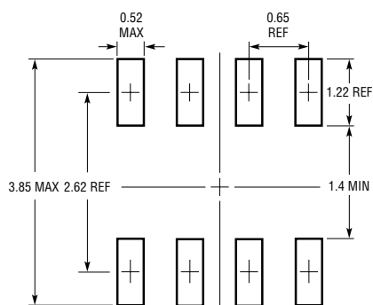
RECOMMENDED SOLDER PAD LAYOUT PER IPC CALCULATOR
