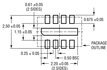
RECOMMENDED SOLDER PAD PITCH AND DIMENSIONS
