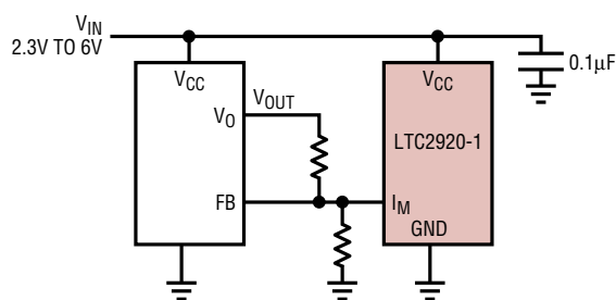
Figure 13. Connecting LTC2920-1 to V_{IN}
