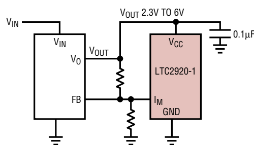
Figure 14. Connecting LTC2920-1 to V_{OUT}
