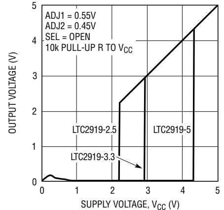
OUT1, OUT2, \overline{\text{RST}} Output Voltage vs V_{CC}
