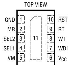
DDB PACKAGE 10-LEAD (3mm \times 2mm) PLASTIC DFN T_{JMAX} = 125^{\circ}\text{C} , \theta_{JA} = 43^{\circ}\text{C/W} EXPOSED PAD (PIN 11) PCB GND CONNECTION OPTIONAL LTC2918
