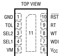
DDB PACKAGE 10-LEAD (3mm \times 2mm) PLASTIC DFN T_{JMAX} = 125^{\circ}\text{C} , \theta_{JA} = 43^{\circ}\text{C/W} EXPOSED PAD (PIN 11) PCB GND CONNECTION OPTIONAL LTC2917
