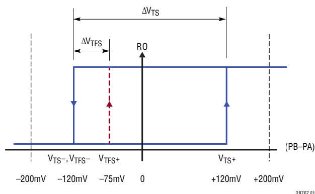
Figure 13. The LTC2876/LTC2877 Signal Thresholds ( V_{TS-} , V_{TS+} ) and Failsafe Thresholds ( V_{TES-} , V_{TES+} )
