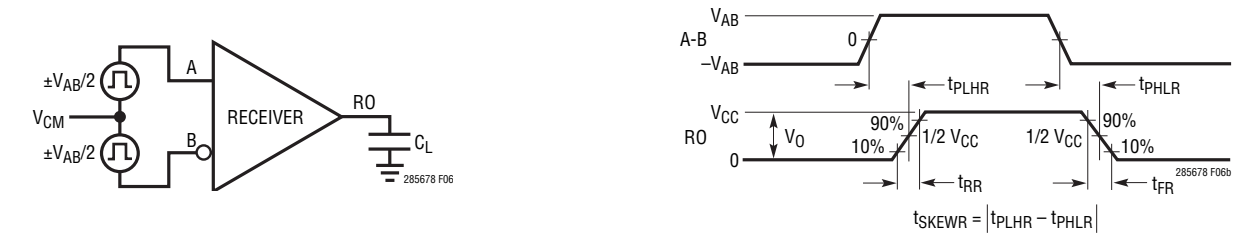
Figure 6. Receiver Propagation Delay Measurements
