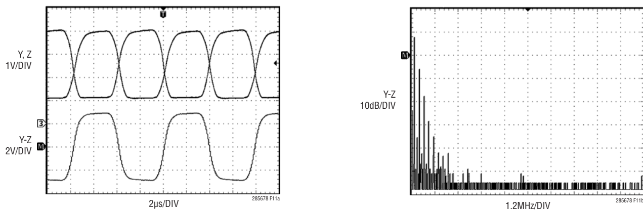
Figure 11. LTC2858-2 Driver Output at 100kHz Into 100Ω Resistor
