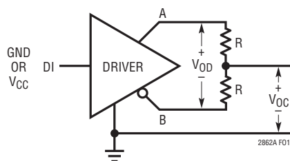
Figure 1. Driver DC Characteristics
