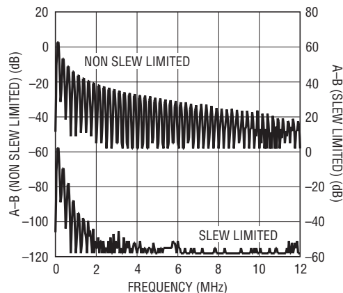
Figure 11. High Frequency EMI Reduction of Slew Limited 250kbps Mode Compared to Non Slew Limited 20Mbps Mode
