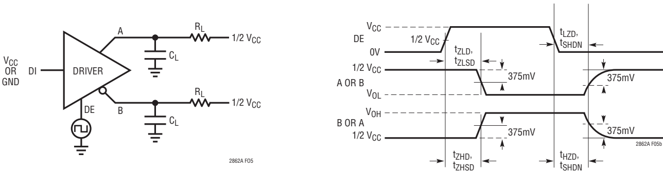
Figure 5. Driver Enable and Disable Timing Measurements
