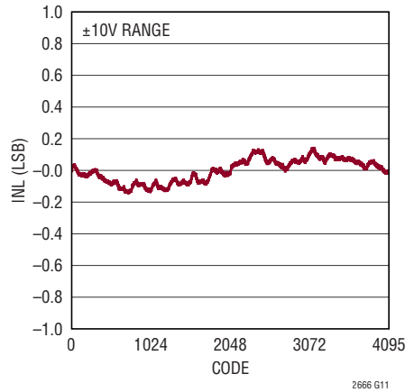
Integral Nonlinearity (INL) (LTC2666-12)
