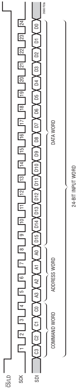
3a. LTC2666-16 24-Bit Load Sequence (Minimum Input Word). LTC2666-12 SDI Input Code + 4 Don't-Care Bits
