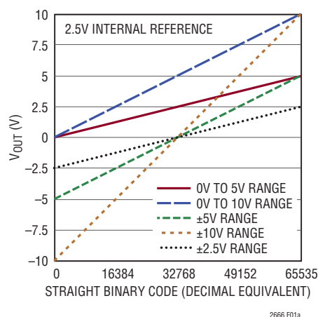
Figure 2a. LTC2666-16 Transfer Function
