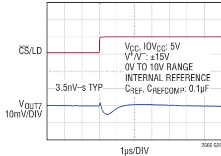
DAC-to-DAC Crosstalk
