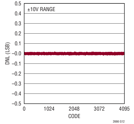
Differential Nonlinearity (DNL) (LTC2666-12)
