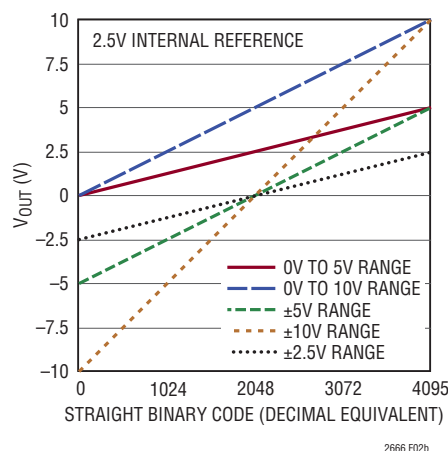
Figure 2b. LTC2666-12 Transfer Function
