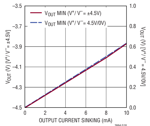
Minimum Output Voltage V_{\text{OUT}} vs Load Current
