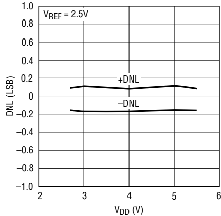
Differential Nonlinearity (DNL) vs Supply ( V_{DD} )
