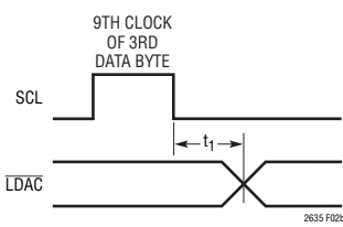
Figure 2b. LTC2635 \overline{\text{LDAC}} Timing (QFN Package Only)
