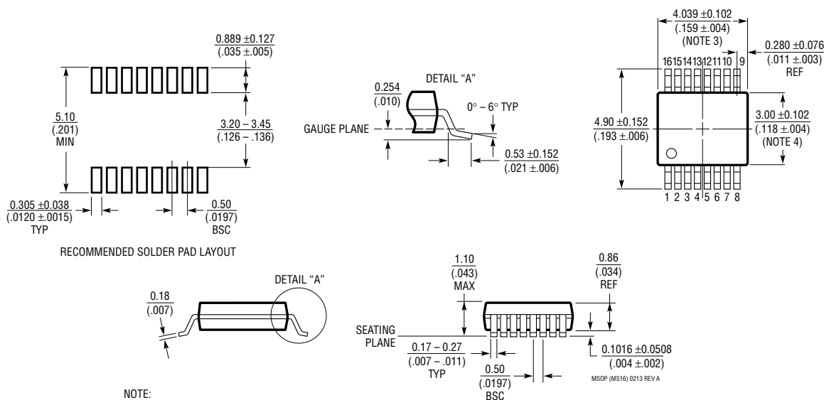
MS Package 16-Lead Plastic MSOP (Reference LTC DWG # 05-08-1669 Rev A)
