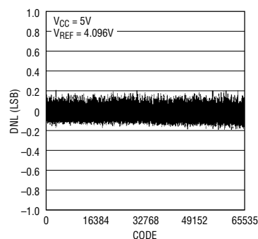
Differential Nonlinearity (LTC2606)
