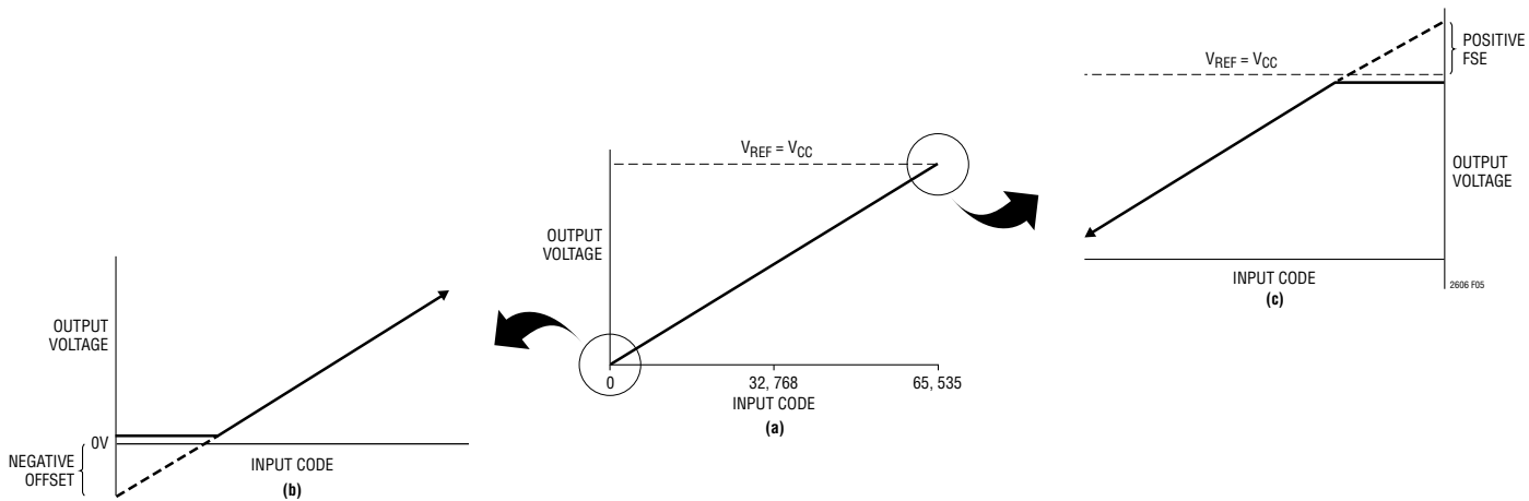
Figure 5. Effects of Rail-to-Rail Operation on a DAC Transfer Curve. (a) Overall Transfer Function (b) Effect of Negative Offset for Codes Near Zero Scale (c) Effect of Positive Full-Scale Error for Codes Near Full Scale
