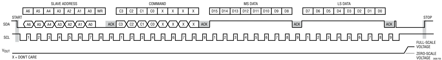
Figure 4. Typical LTC2606 Input Waveform—Programming DAC Output for Full Scale
