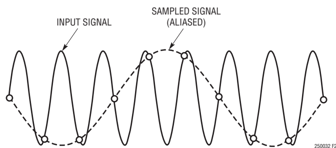
Figure 22. Time Domain View of Aliasing
