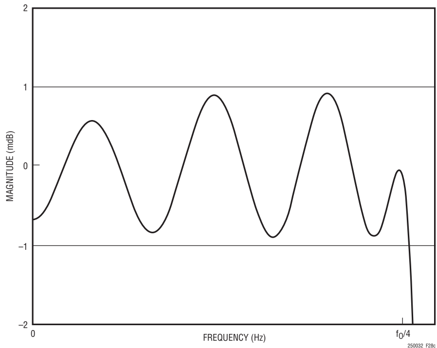
Figure 28c. Low Ripple Passband Portion of Frequency Response from Figure 28b
