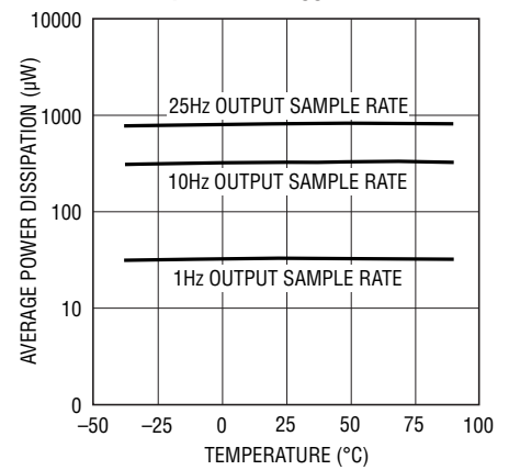
Average Power Dissipation vs Temperature, V_{CC} = 3V
