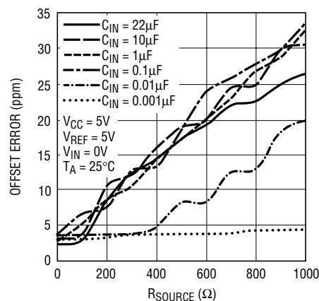
Figure 21. Offset vs R_{SOURCE} (Large C)
