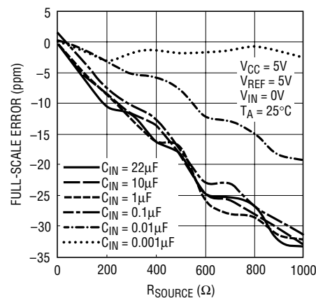
Figure 22. Full-Scale Error vs R_{SOURCE} (Large C)
