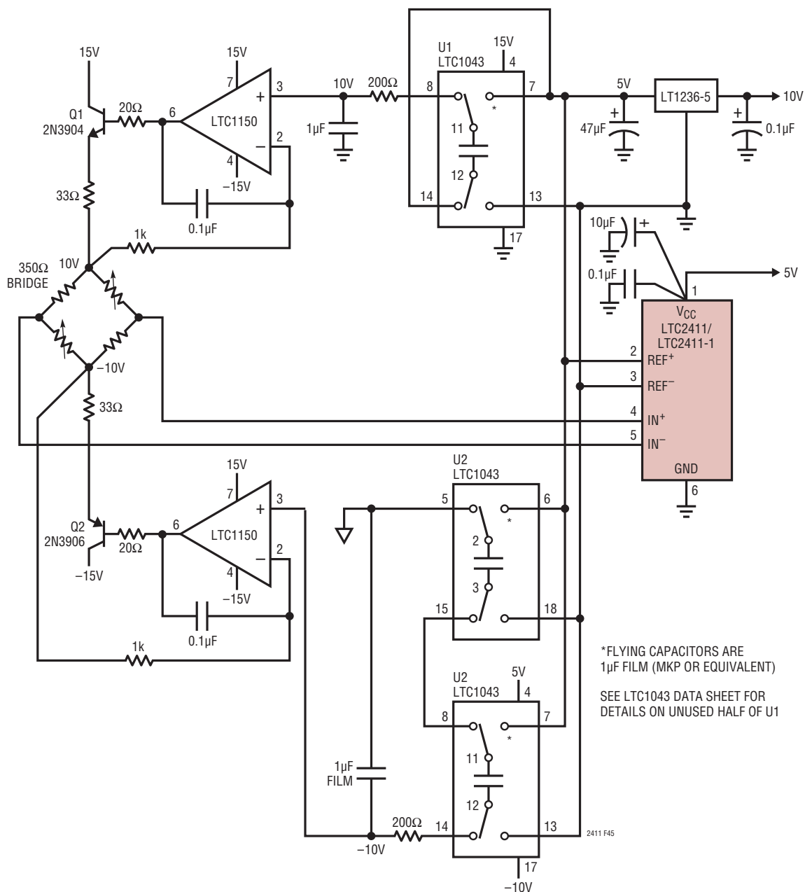
Figure 45. LTC1043 Provides Precise 4 \times Reference for Excitation Voltages
