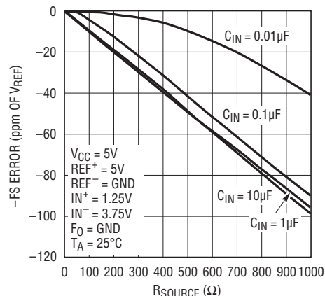
Figure 15b. ^-\text{FS} Error vs R_{\text{SOURCE}} at \text{IN}^+ or \text{IN}^- (Large C_{\text{IN}} )
