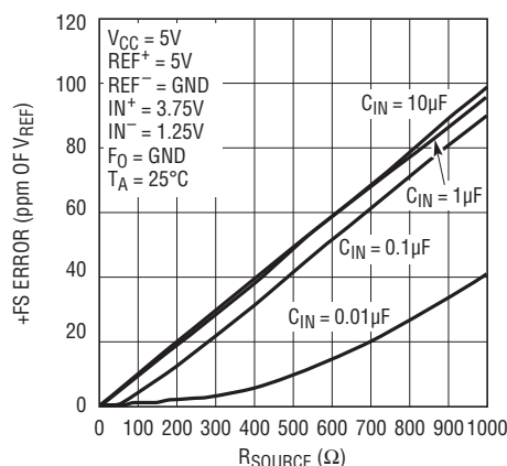
Figure 15a. ^+\text{FS} Error vs R_{\text{SOURCE}} at \text{IN}^+ or \text{IN}^- (Large C_{\text{IN}} )
