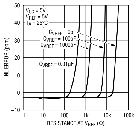
Figure 24. INL Error vs R_{VREF} (Small C)
