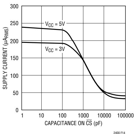
Figure 14. \overline{\text{CS}} Capacitance vs Supply Current
