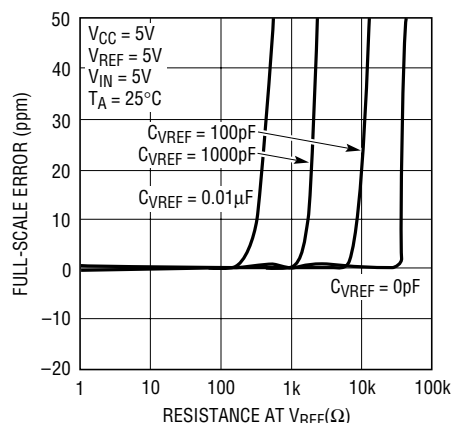
Figure 23. Full-Scale Error vs R_{VREF} (Small C)
