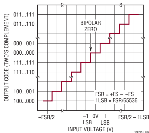
Figure 2. LTC2389-16 Two's Complement Transfer Function. Offset Binary Transfer Function Can Be Obtained by Inverting the Most Significant Bit (MSB) of Each Output Code
