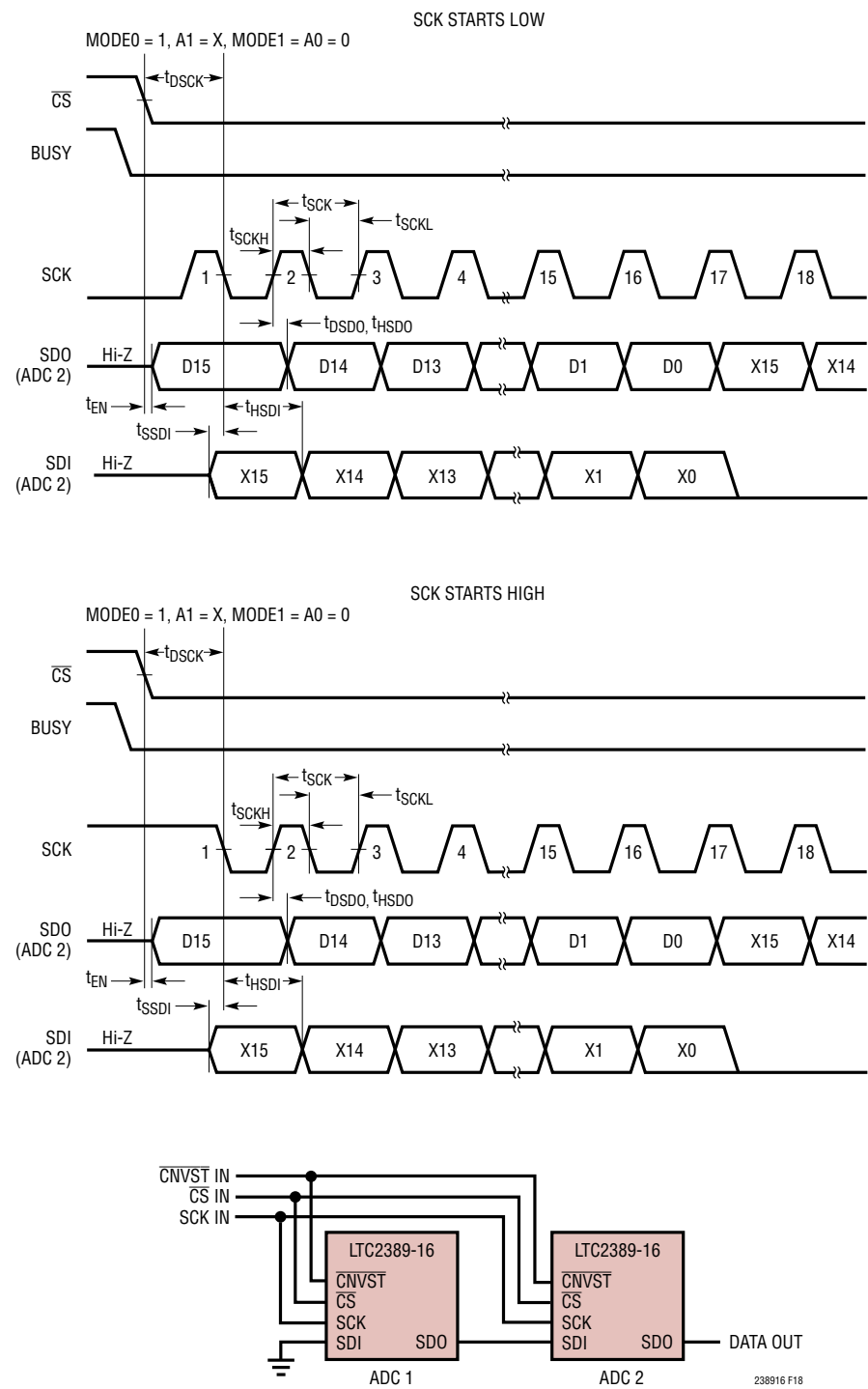
Figure 18. Serial Interface with External Clock. Read After the Conversion. Daisy Chain Multiple Converters
