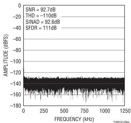
Figure 6d. 32k Point FFT f_{\text{SMPL}} = 2.5\text{Msps} , f_{\text{IN}} = 2\text{kHz} , for Circuit Shown in Figure 6a; Driven with Bipolar Inputs
