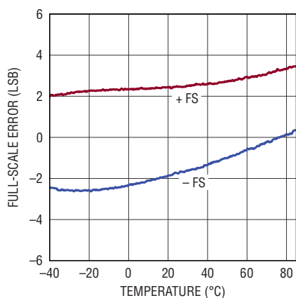
Full-Scale Error vs Temperature, REFBUF = 4.096V
