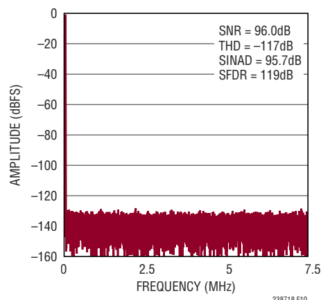
Figure 10. 32k Point FFT of the LTC2387-18, f_{\text{SMPL}} = 15\text{Msps} , f_{\text{IN}} = 2\text{kHz}
