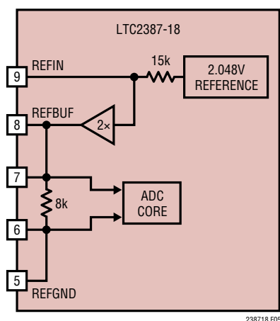
Figure 5. LTC2387-18 Internal Reference Circuitry
