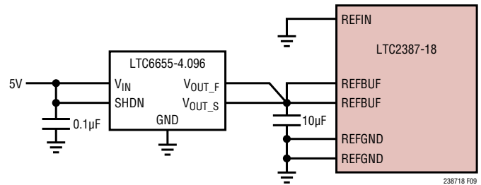
Figure 9. Overdriving REFBUF Using the LTC6655-4.096
